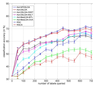
Figure 2: ACM Conference Learning Curves
