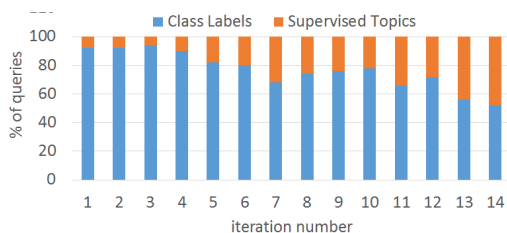
Figure 3: aYahoo Query Distribution
