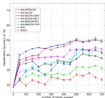
Figure 1: aYahoo Learning Curves
