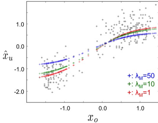
Figure 3: Old Faithful dataset. The original dataset is plotted using black ‘+’. The imputed features with various \lambda_M ’s are shown in different colors. All features are standardized centered at zero.
