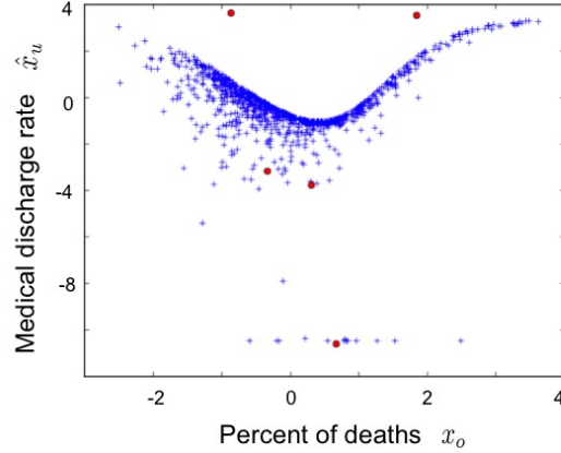
Figure 5: Imputed Dartmouth Dataset at Hospital-level ( K = 5 ). Cluster centroids are plotted using red dots. Horizontal axis shows ‘Percent of death occurring in hospital’ and vertical axis indicates the imputed ‘Medical discharge rate’ at hospital-level. All features are standardized. (Case 1)
