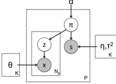
Figure 2: Graphical Model of CUDIA.
